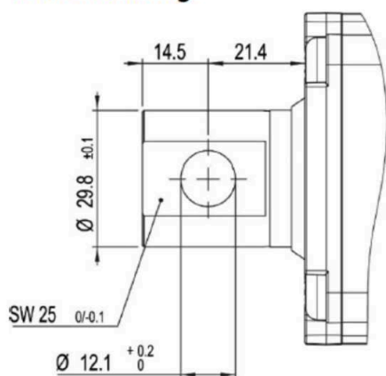
Front mounting:
