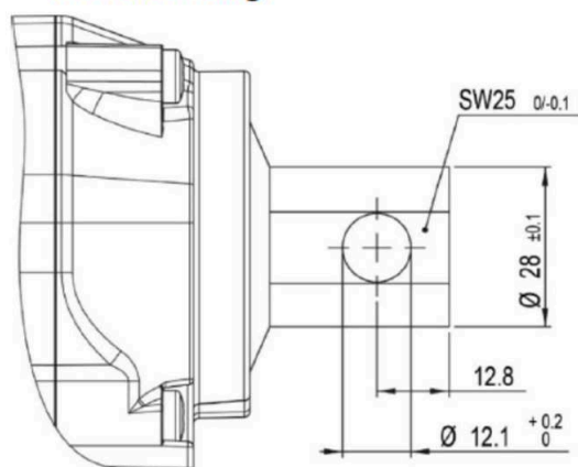
Rear mounting:
