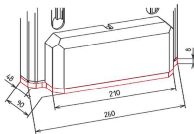
Compression plate
