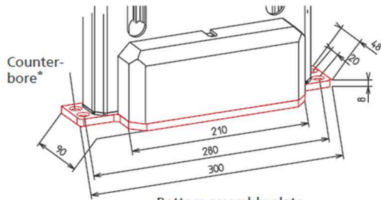
Bottom assembly plate with 4 counterbores
