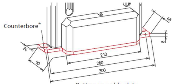
Bottom assembly plate with 2 counterbores
