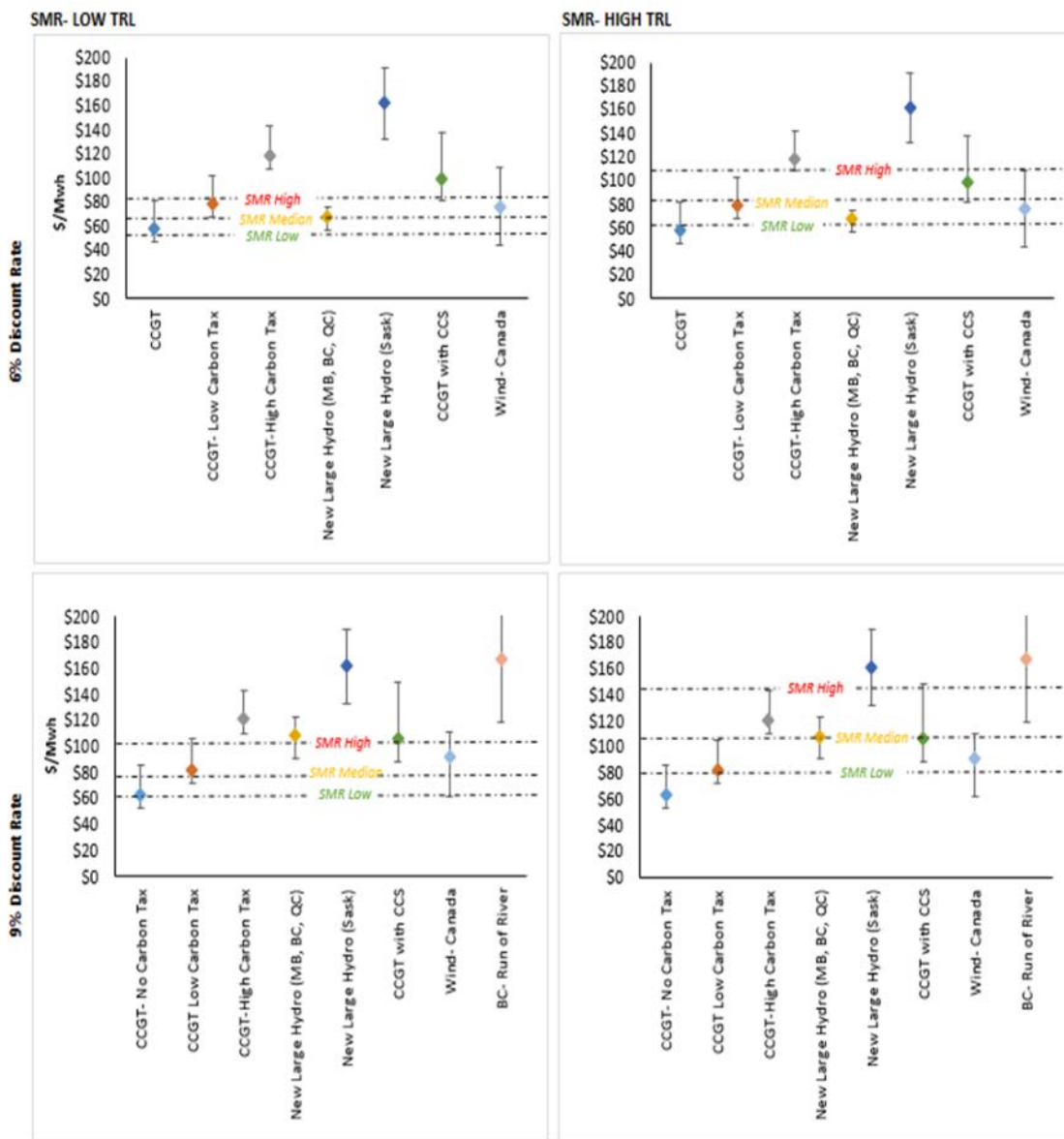
Figure 10 On-grid LCOE at 6% and 9% discount rates
